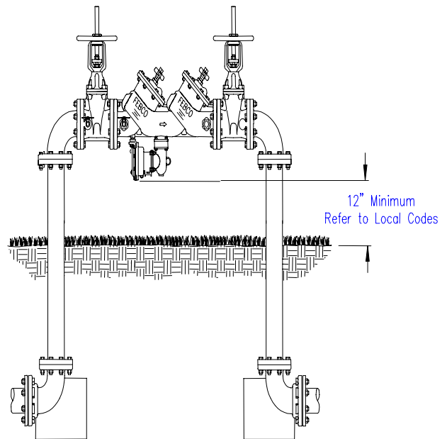
Reduced Pressure Assembly Outdoor Installation -OS&Y Gates
